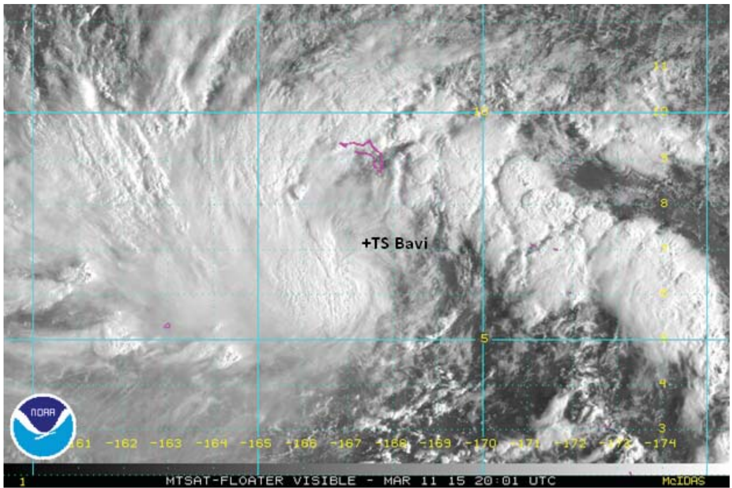
An MTSAT-2 Visible Satellite image of Tropical Storm Bavi, taken at 8:01 a.m., March 12.
