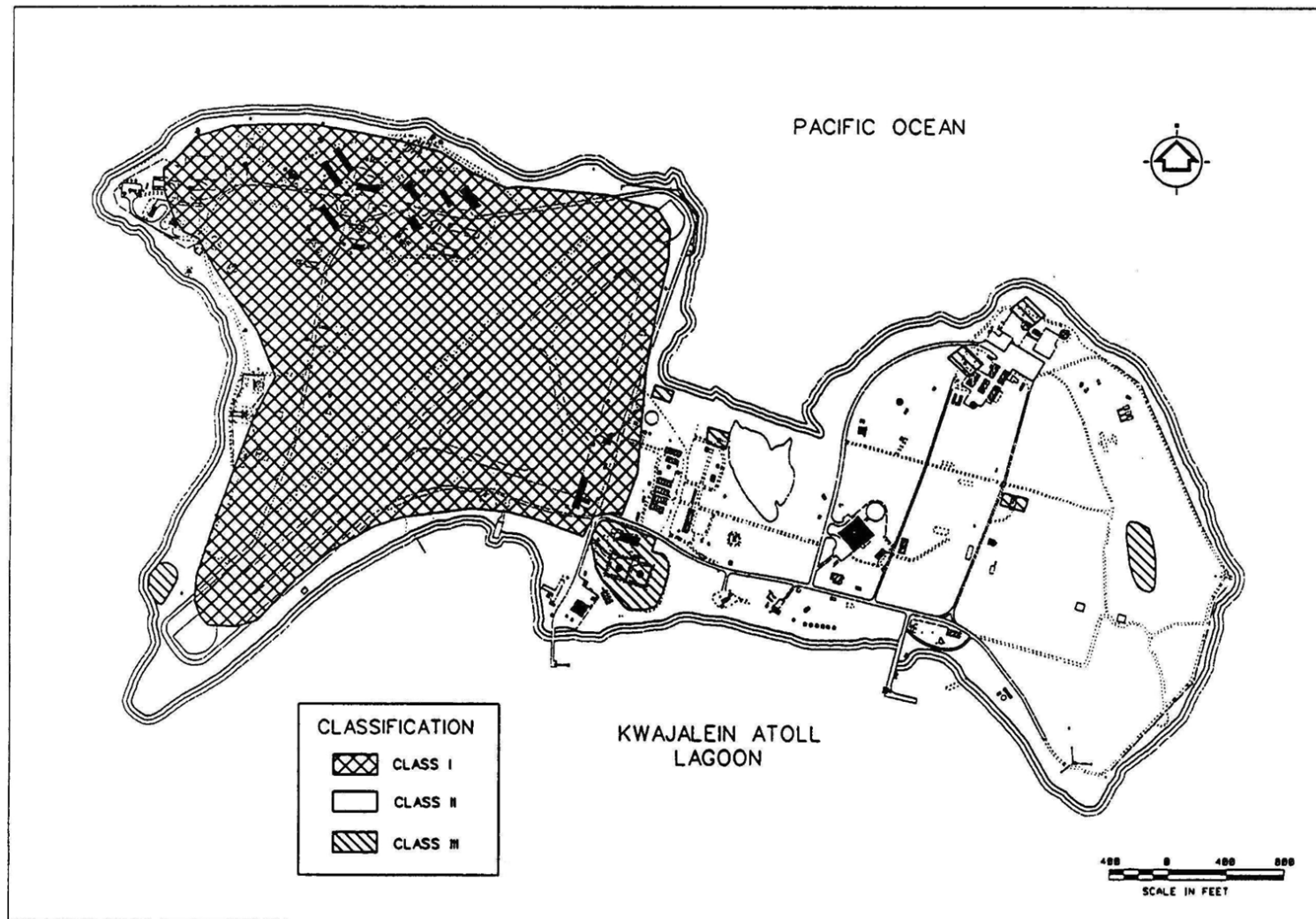
FIGURE 3-2B.2 GROUNDWATER CLASSIFICATION FOR ROI-NAMUR
