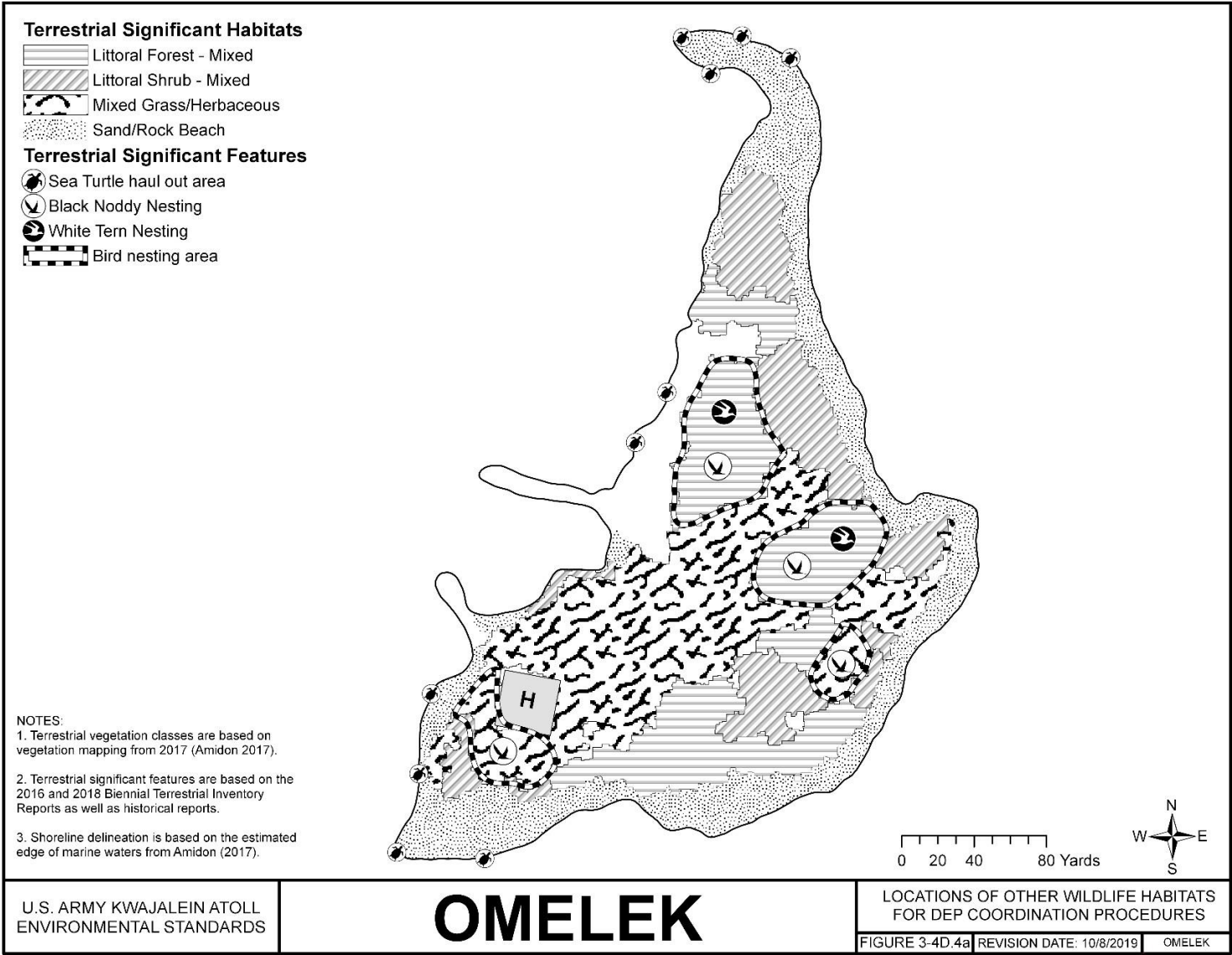
FIGURE 3-4D.4A OMELEK – LOCATIONS OF OTHER WILDLIFE HABITATS FOR DEP COORDINATION PROCEDURES; TERRESTRIAL
