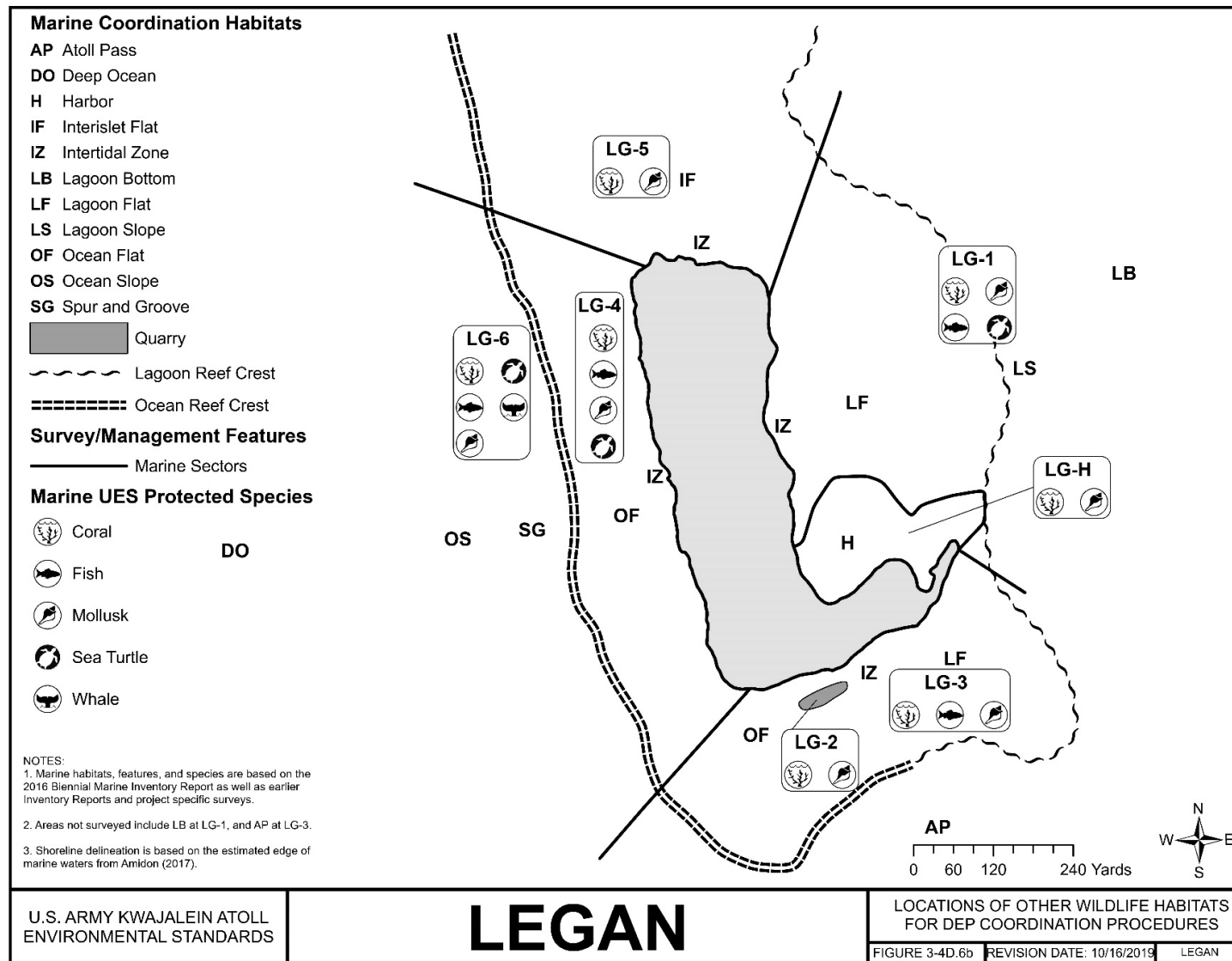
FIGURE 3-4D.6B LEGAN – LOCATIONS OF OTHER WILDLIFE HABITATS FOR DEP COORDINATION PROCEDURES; MARINE
