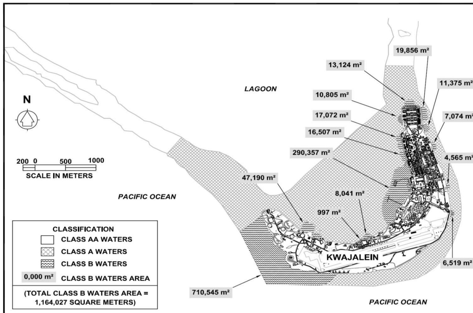
FIGURE 3-2A.1 KWAJALEIN VICINITY: CLASSIFICATION OF COASTAL WATER USE
