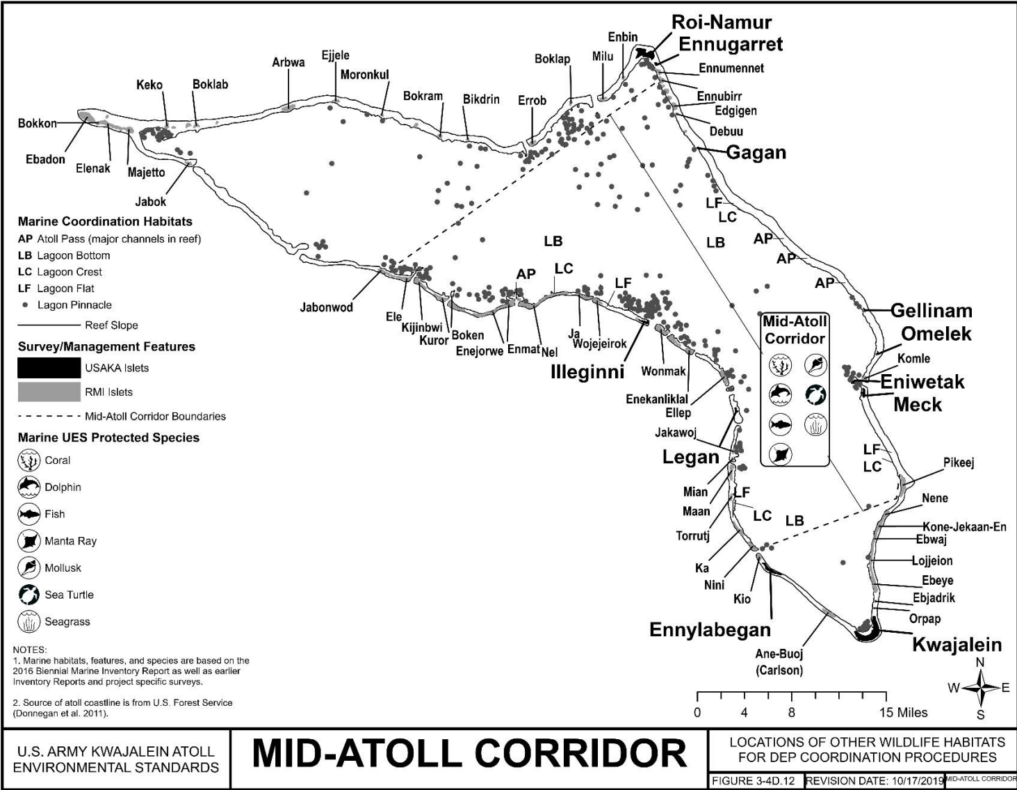
FIGURE 3-4D.12 MID-ATOLL CORRIDOR – LOCATIONS OF OTHER WILDLIFE HABITATS FOR DEP COORDINATION PROCEDURES; MARINE
