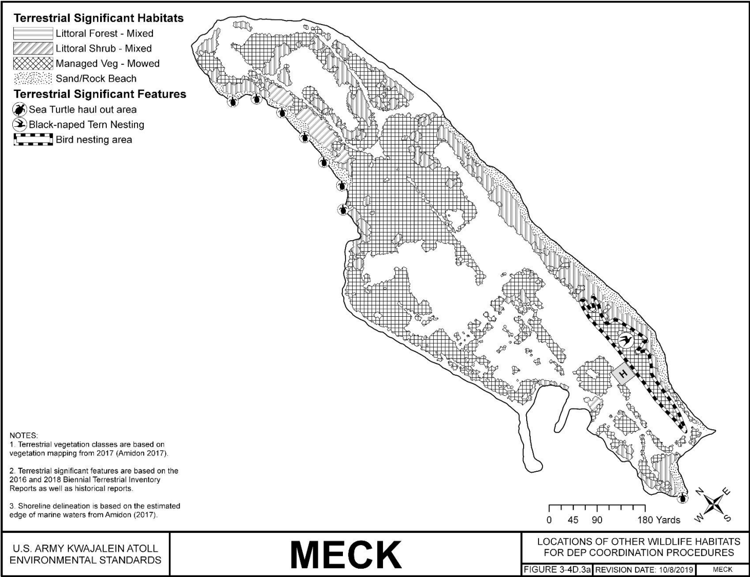
FIGURE 3-4D.3A MECK – LOCATIONS OF OTHER WILDLIFE HABITATS FOR DEP COORDINATION PROCEDURES; TERRESTRIAL
