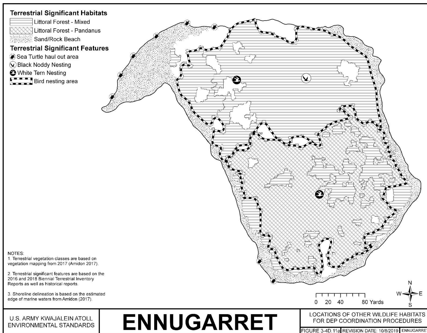
FIGURE 3-4D.11A ENNUGARRET - LOCATIONS OF OTHER HABITATS FOR DEP COORDINATION PROCEDURES; TERRESTRIAL
