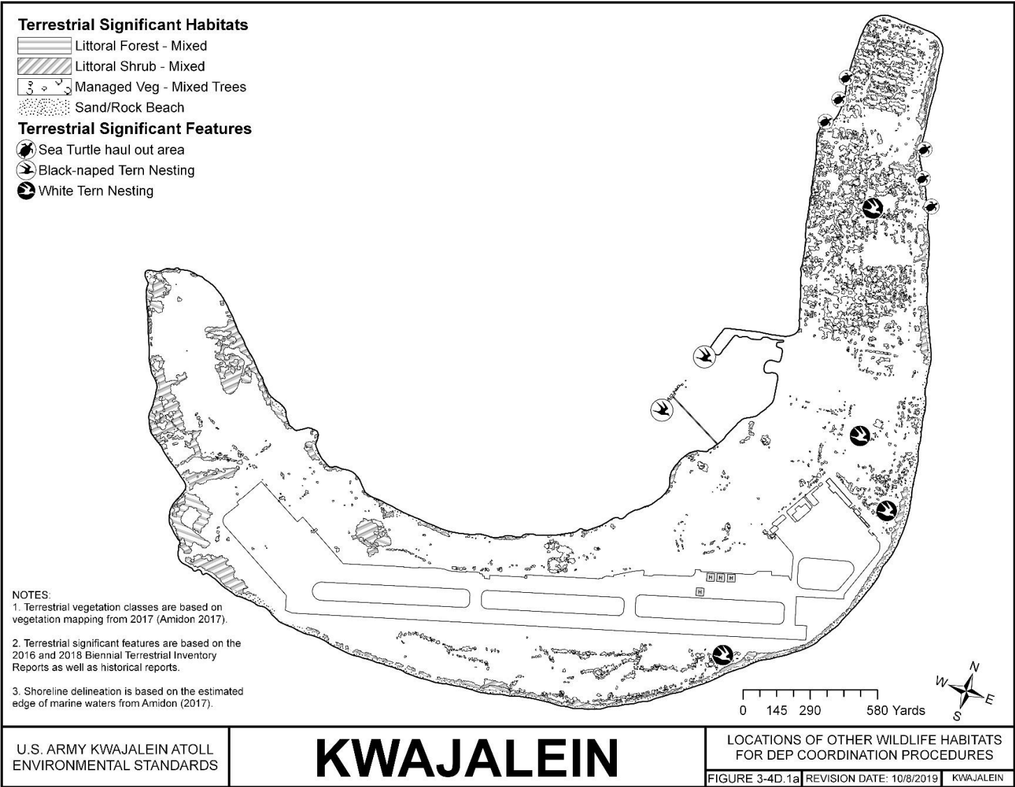
FIGURE 3-4D.1A KWAJALEIN – LOCATIONS OF OTHER WILDLIFE HABITATS FOR DEP COORDINATION PROCEDURES; TERRESTRIAL
