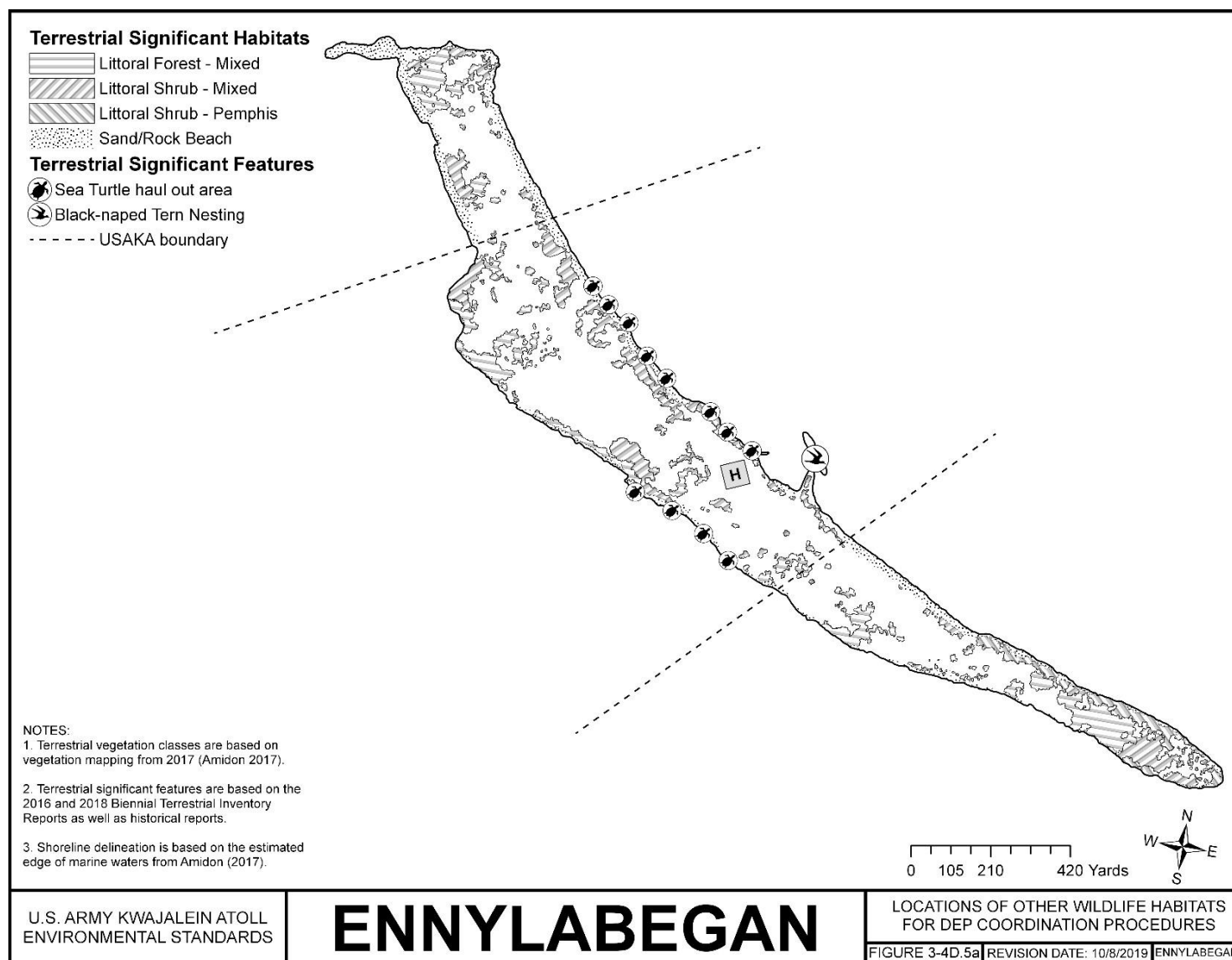
FIGURE 3-4D.5A ENNYLABEGAN – LOCATIONS OF OTHER WILDLIFE HABITATS FOR DEP COORDINATION PROCEDURES; TERRESTRIAL
