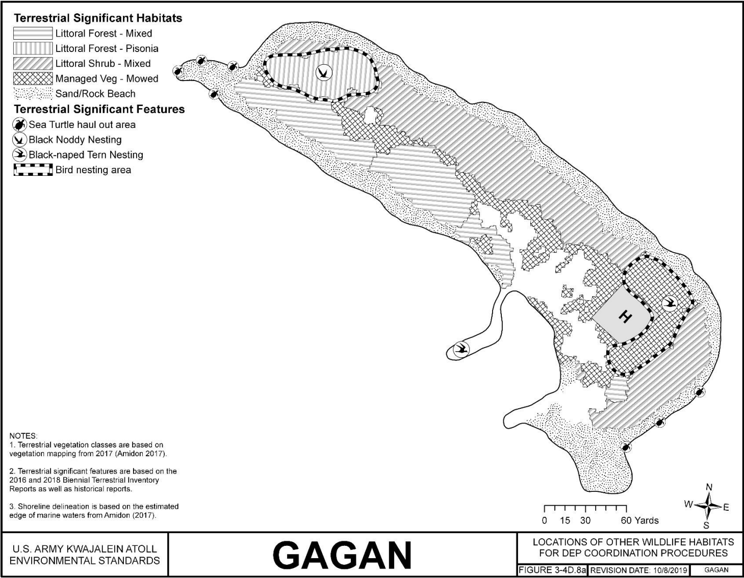
FIGURE 3-4D.8A GAGAN – LOCATIONS OF OTHER WILDLIFE HABITATS FOR DEP COORDINATION PROCEDURES; TERRESTRIAL
