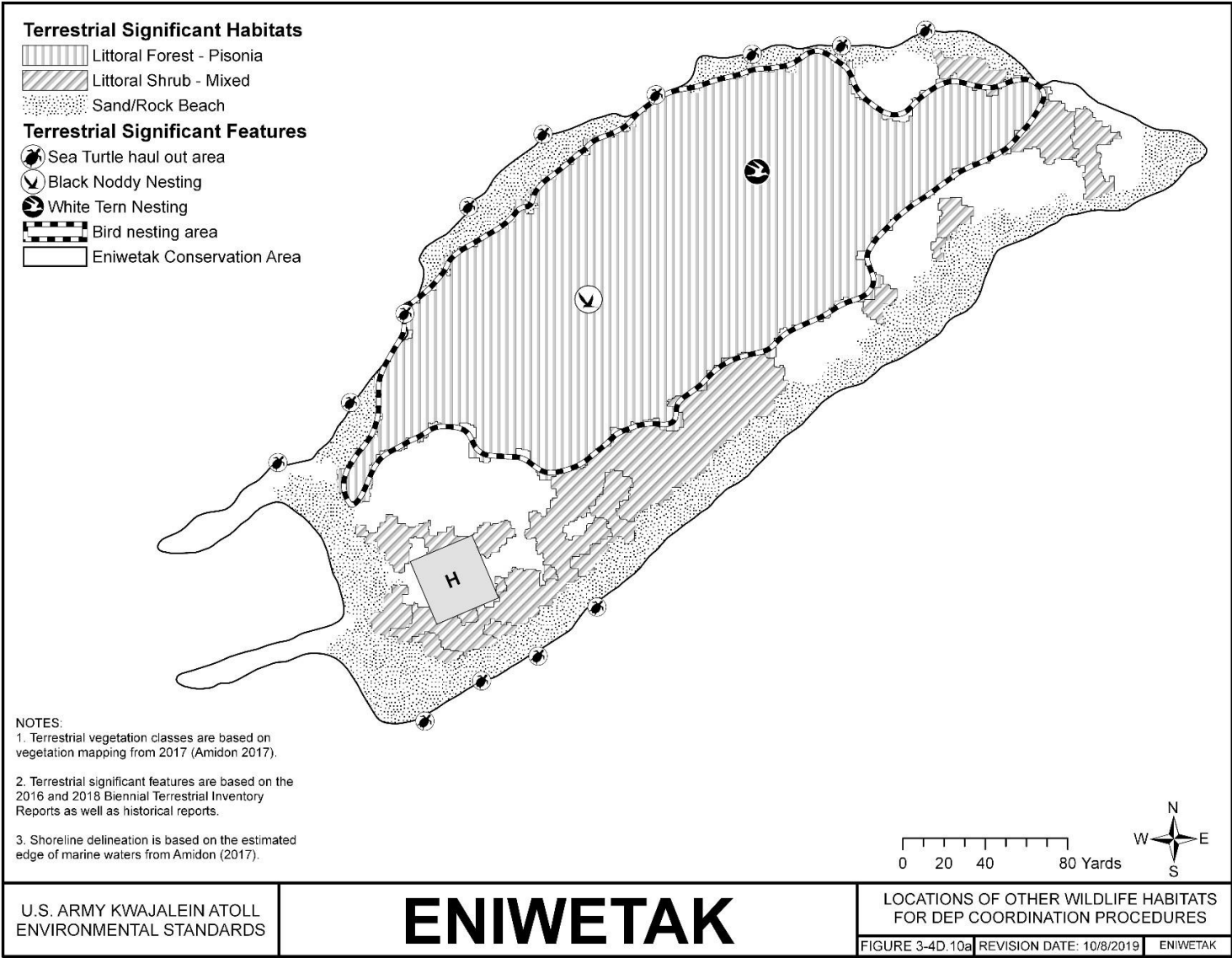
FIGURE 3-4D.10A ENIWETAK - LOCATIONS OF OTHER WILDLIFE HABITATS FOR DEP COORDINATION PROCEDURES; TERRESTRIAL
