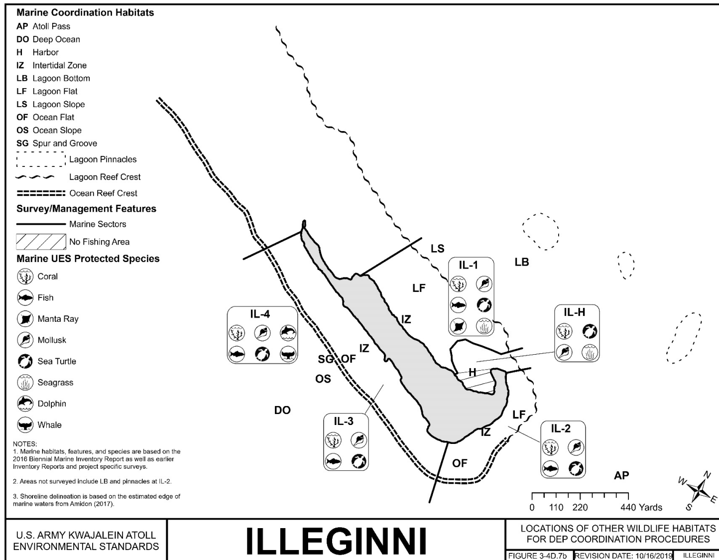
FIGURE 3-4D.7B ILLEGINNI – LOCATIONS OF OTHER WILDLIFE HABITATS FOR DEP COORDINATION PROCEDURES; MARINE
