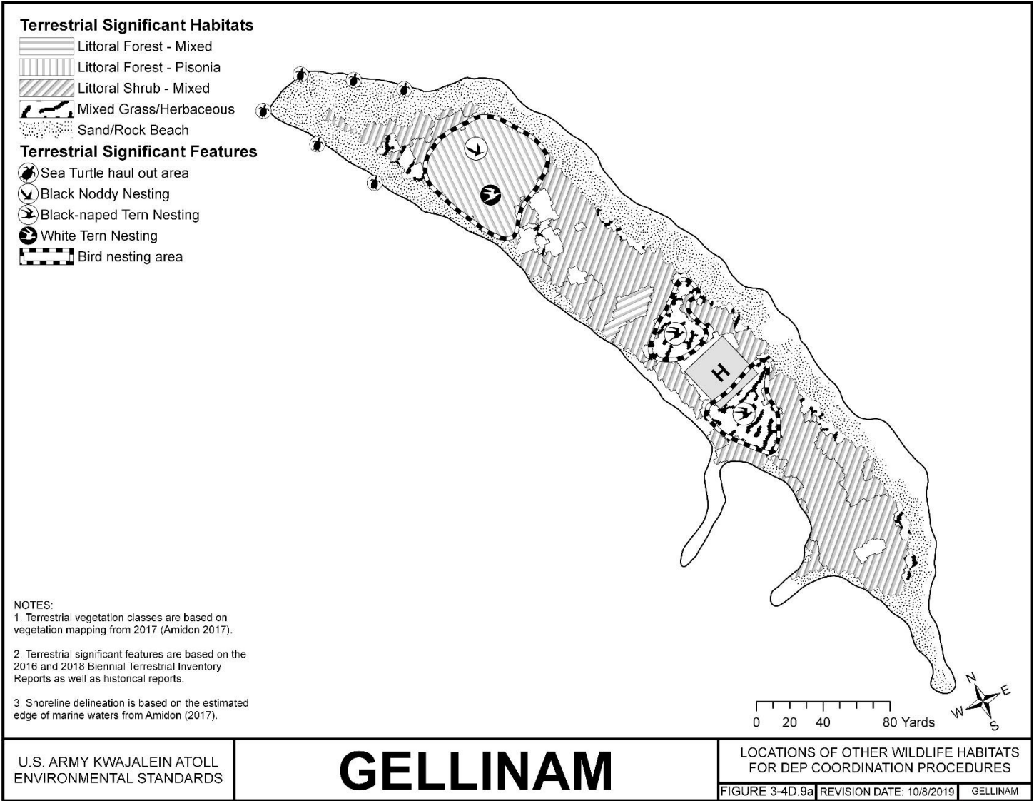
FIGURE 3-4D.9A GELLINAM – LOCATIONS OF OTHER WILDLIFE HABITATS FOR DEP COORDINATION PROCEDURES; TERRESTRIAL
