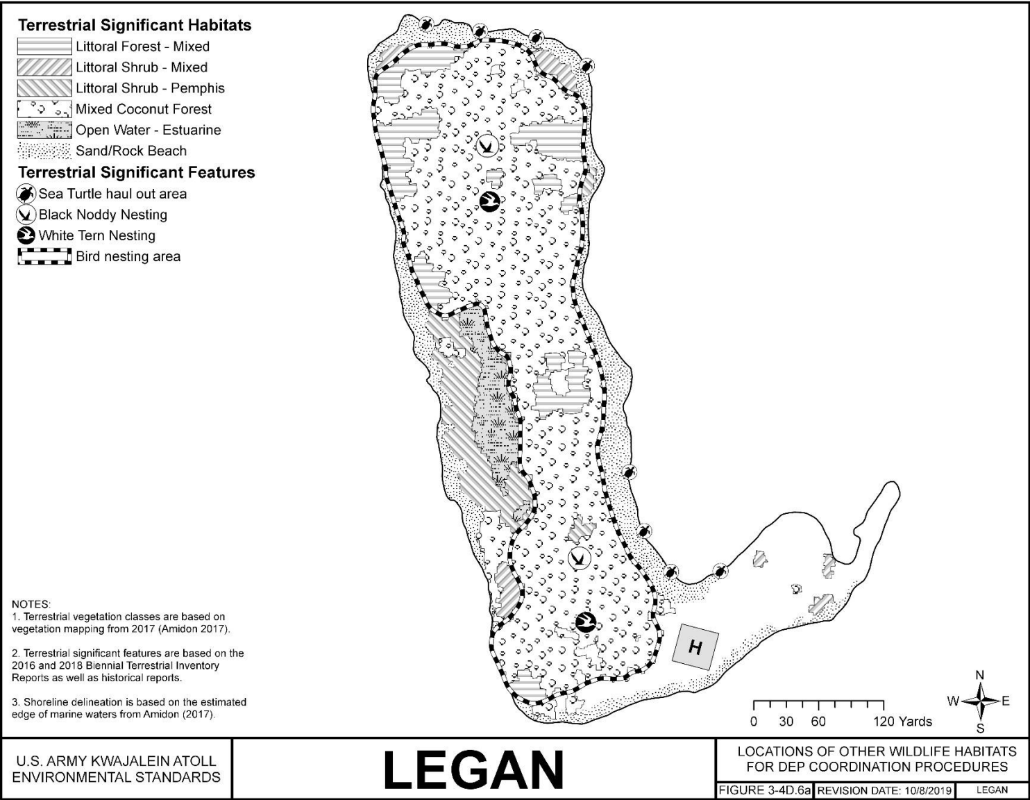
FIGURE 3-4D.6A LEGAN – LOCATIONS OF OTHER WILDLIFE HABITATS FOR DEP COORDINATION PROCEDURES; TERRESTRIAL
