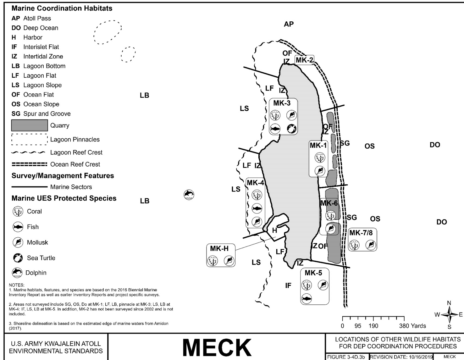
FIGURE 3-4D.3B MECK – LOCATIONS OF OTHER WILDLIFE HABITATS FOR DEP COORDINATION PROCEDURES; MARINE
