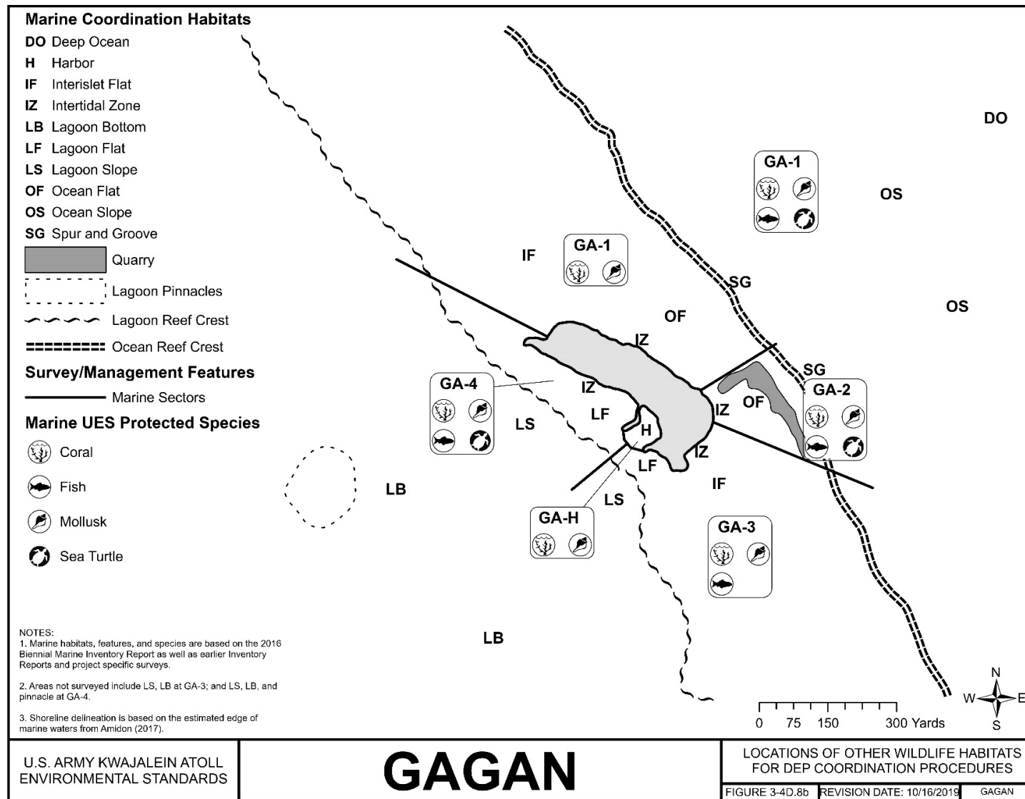
FIGURE 3-4D.8B GAGAN – LOCATIONS OF OTHER WILDLIFE HABITATS FOR DEP COORDINATION PROCEDURES; MARINE
