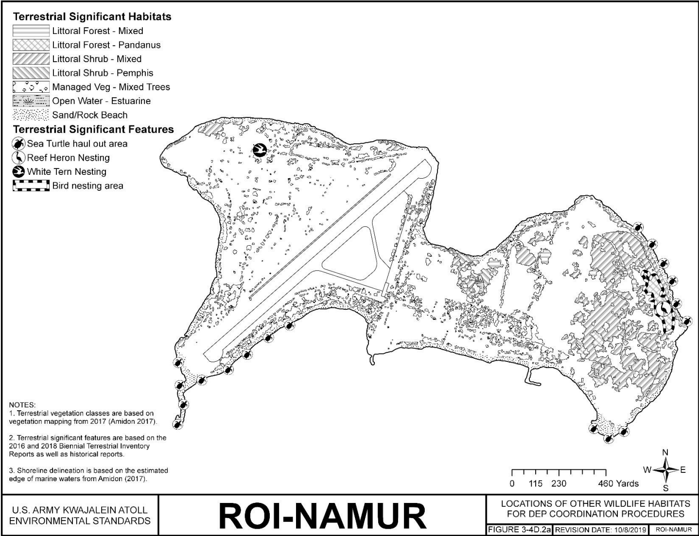
FIGURE 3-4D.2A ROI-NAMUR – LOCATIONS OF OTHER WILDLIFE HABITATS FOR DEP COORDINATION PROCEDURES; TERRESTRIAL
