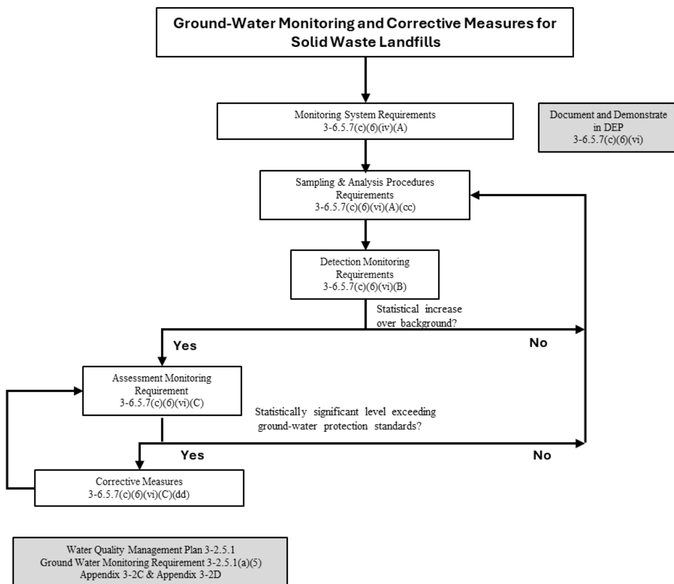
FIGURE 3-6.1.11 GROUND-WATER MONITORING AND CORRECTIVE MEASURES FOR SOLID WASTE LANDFILLS
