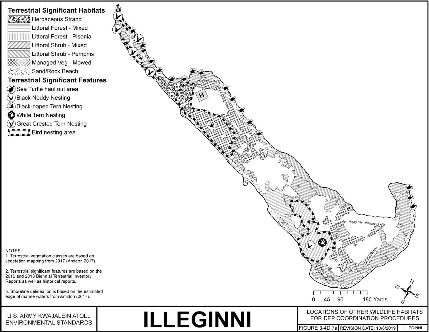
FIGURE 3-4D.7A ILLEGINNI – LOCATIONS OF OTHER WILDLIFE HABITATS FOR DEP COORDINATION PROCEDURES; TERRESTRIAL
