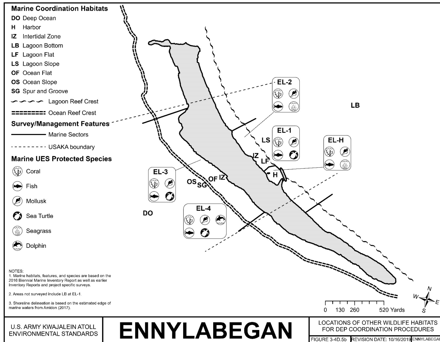
FIGURE 3-4D.5B ENNYLABEGAN – LOCATIONS OF OTHER WILDLIFE HABITATS FOR DEP COORDINATION PROCEDURES; MARINE
