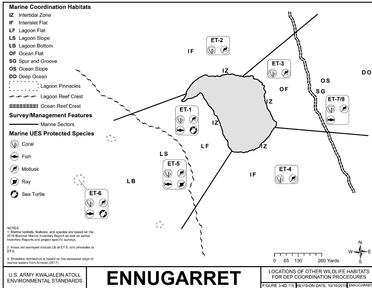
FIGURE 3-4D.11B ENUGARRET – LOCATIONS OF OTHER WILDLIFE HABITATS FOR DEP COORDINATION PROCEDURES; MARINE
