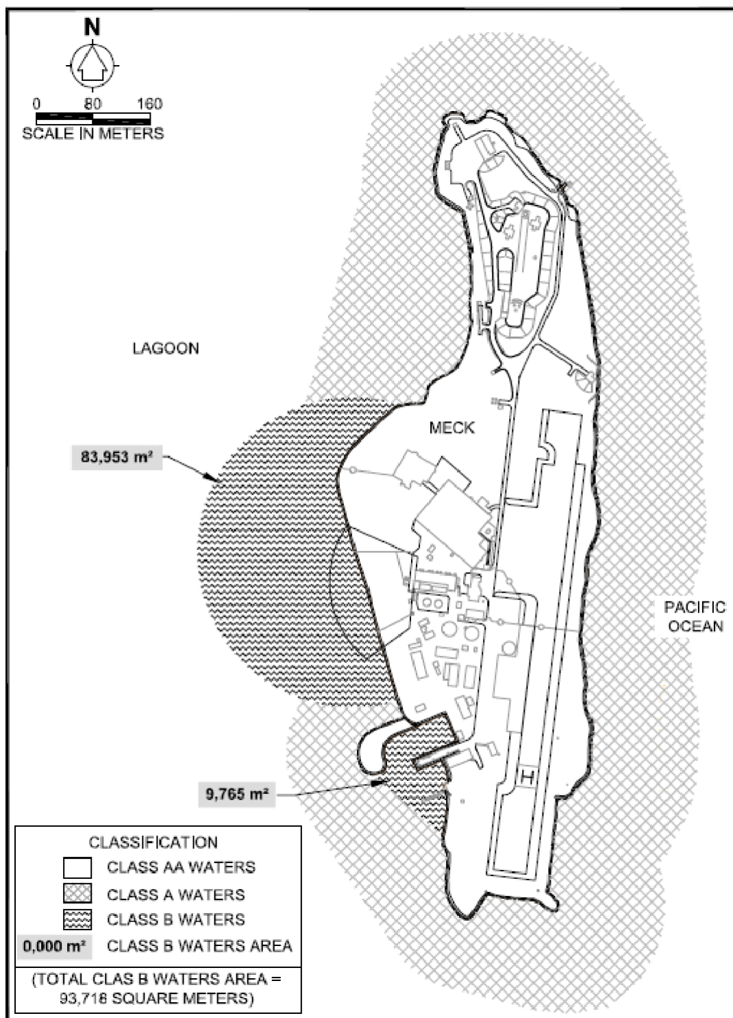
FIGURE 3-2A.3 MECK VICINITY: CLASSIFICATION OF COASTAL WATER USE
