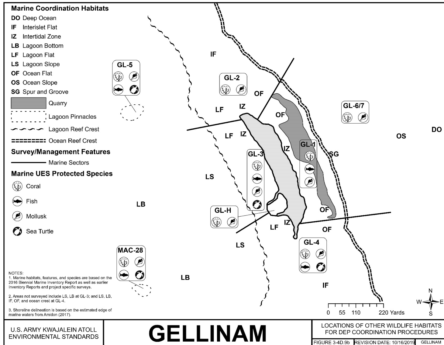
FIGURE 3-4D.9B GELLINAM – LOCATIONS OF OTHER WILDLIFE HABITATS FOR DEP COORDINATION PROCEDURES; MARINE
