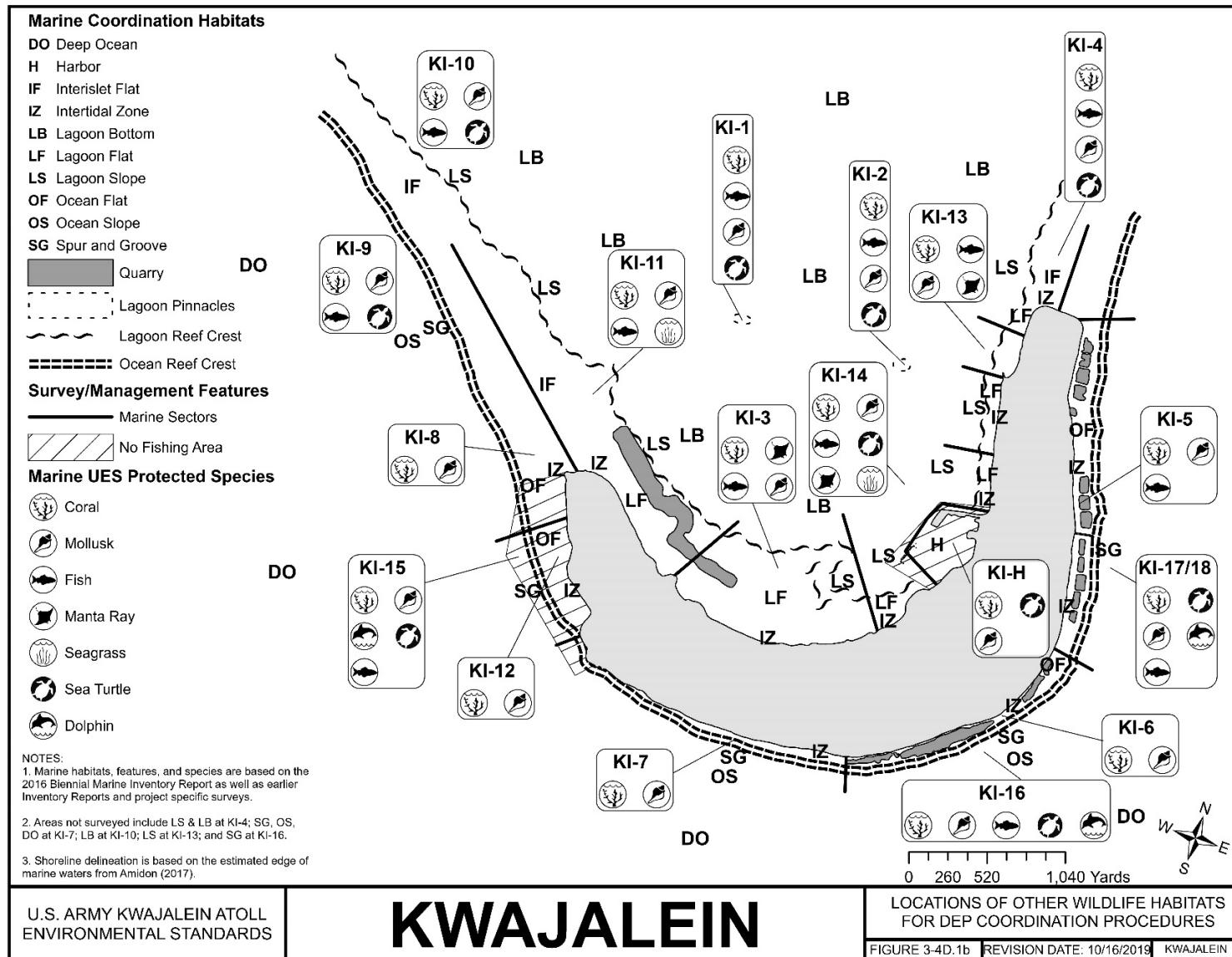
FIGURE 3-4D.1B KWAJALEIN – LOCATIONS OF OTHER WILDLIFE HABITATS FOR DEP COORDINATION PROCEDURES; MARINE
