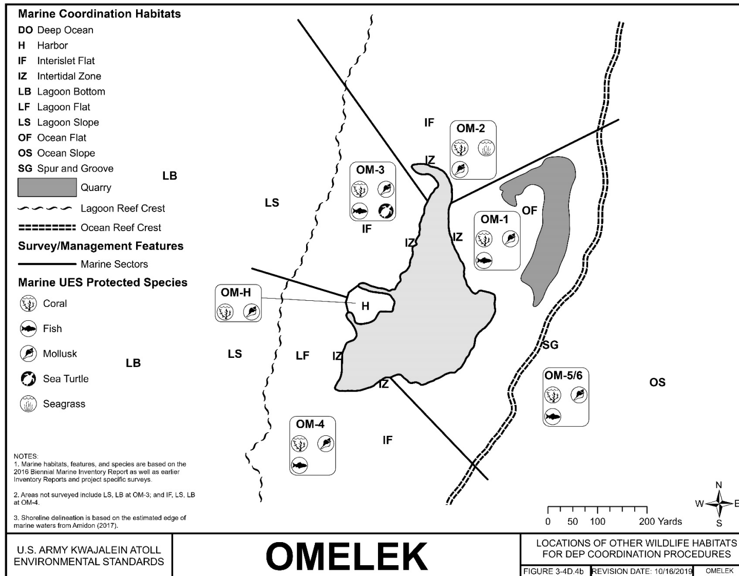
FIGURE 3-4D.4B OMELEK – LOCATIONS OF OTHER WILDLIFE HABITATS FOR DEP COORDINATION PROCEDURES; MARINE
