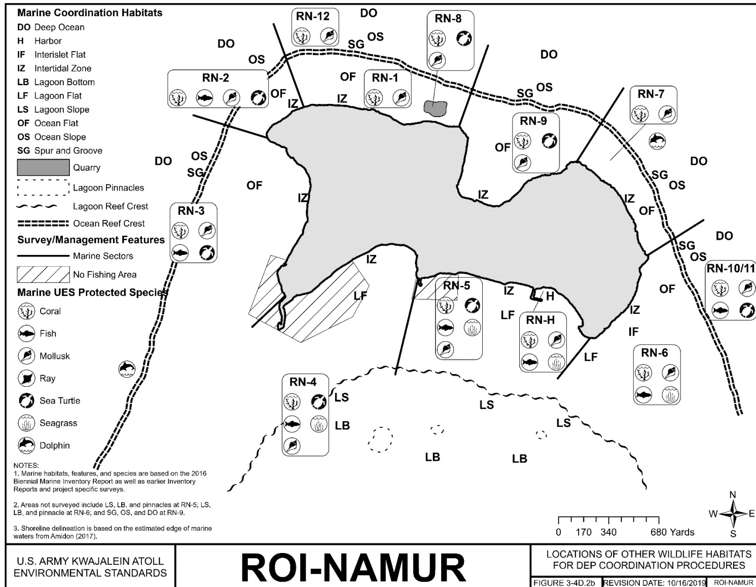
FIGURE 3-4D.2B ROI-NAMUR – LOCATIONS OF OTHER WILDLIFE HABITATS FOR DEP COORDINATION PROCEDURES; MARINE
