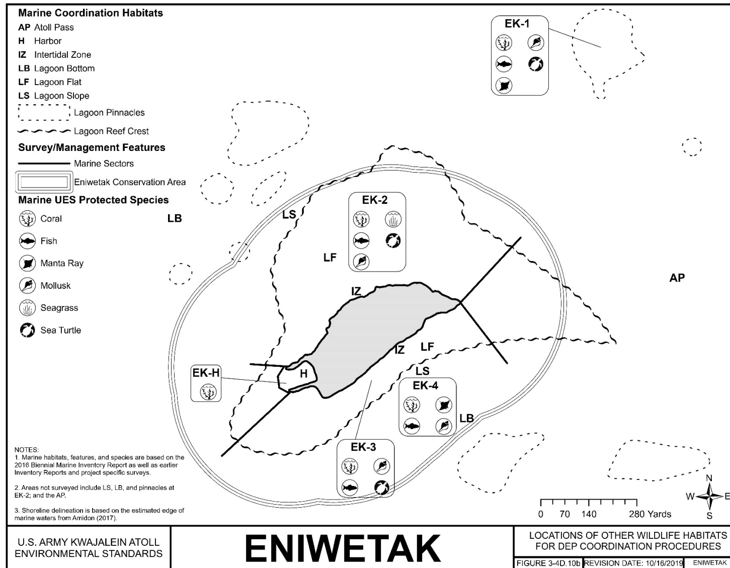
FIGURE 3-4D.10B ENIWETAK - LOCATIONS OF OTHER HABITATS FOR DEP COORDINATION PROCEDURES; MARINE
